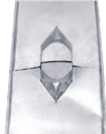
Havalandırma Boru Kenar Sacı Galvanizli Galvanized Side Plates for Ventilation Pipe
